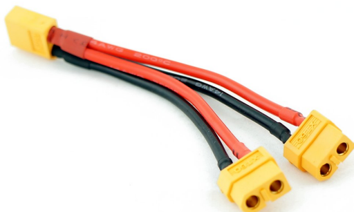
XT60 splitter – XT60 male connector on the left, two XT60 female connectors on the right
